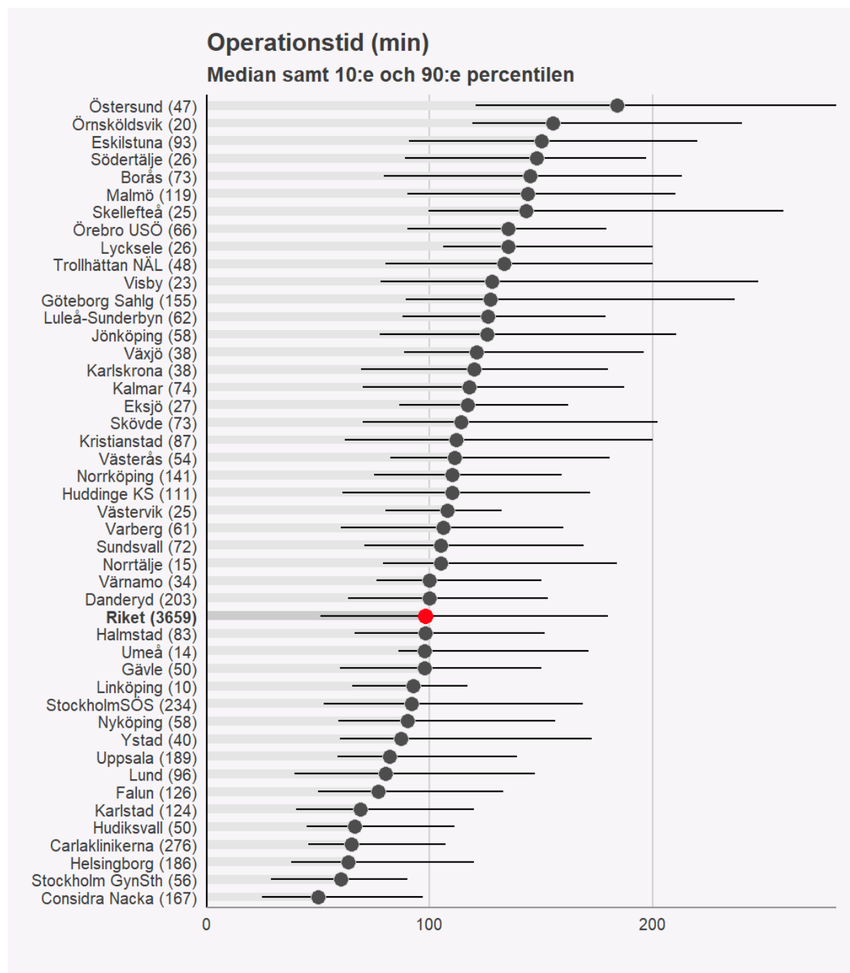
Figur 15. Operationstid (min).
